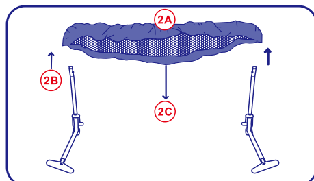
2. A. Insert the top joint pipe through the nylon mesh (A). B. Connect the standing legs (D1 and D2) at both sides of the nylon mesh (A). C. Pull down the nylon mesh (A).
